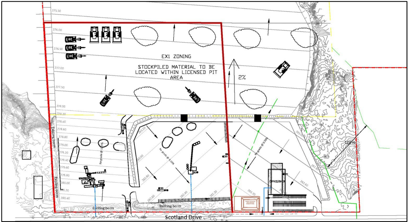
Figure 1. Site Concept Plan for 3696 and 3832 Scotland Drive
